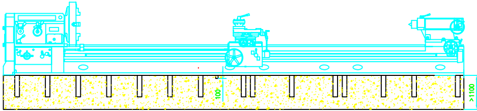
max. workpiece length 12000mm
